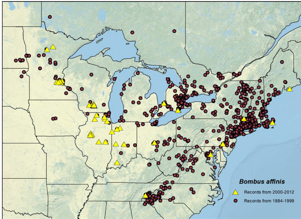
Figure 1. Historic (1884-1999) distribution of the rusty patched bumble bee represented by circles; contemporary (2000-2012) distribution of the rusty patched bumble bee represented by triangles. Note that bumble bee search effort has dramatically increased since 2000 relative to the entire 20 th Century (see Figure 1 in Colla et al. 2012, which uses the same dataset), and many observers have specifically targeted the rusty-patched bumble bee in recent years. Data for this map is from Colla et al. In Prep. Original data sources are listed in Appendix I.
